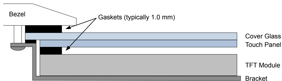
Figure 1: Mounting Diagram
